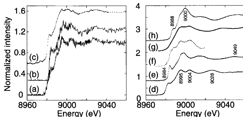
Fig. 4. Site-selective XANES spectra for Cu/ZnO catalyst. Fluorescence spectrometer was tuned to 8046.6 eV (a) and to 8050.9 eV (b). Conventional XANES spectra for Cu/ZnO (c), Cu foil (d), Cu 2 O (e), [Cu(TEPA)][BPh 4 ] (f), and CuO (h) were measured by Lytle detector (c) or in transmission mode (d, e, h). XANES was theoretically generated by FEFF8 for Cu I atomically dispersed on ZnO (g). XANES of [Cu(TEPA)][BPh 4 ] was reproduced from Ref. 13.
